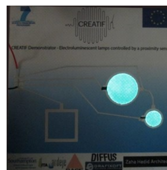
Combined inkjet and smart ink printed images with printed lamps before (top) and after activation (bottom)
